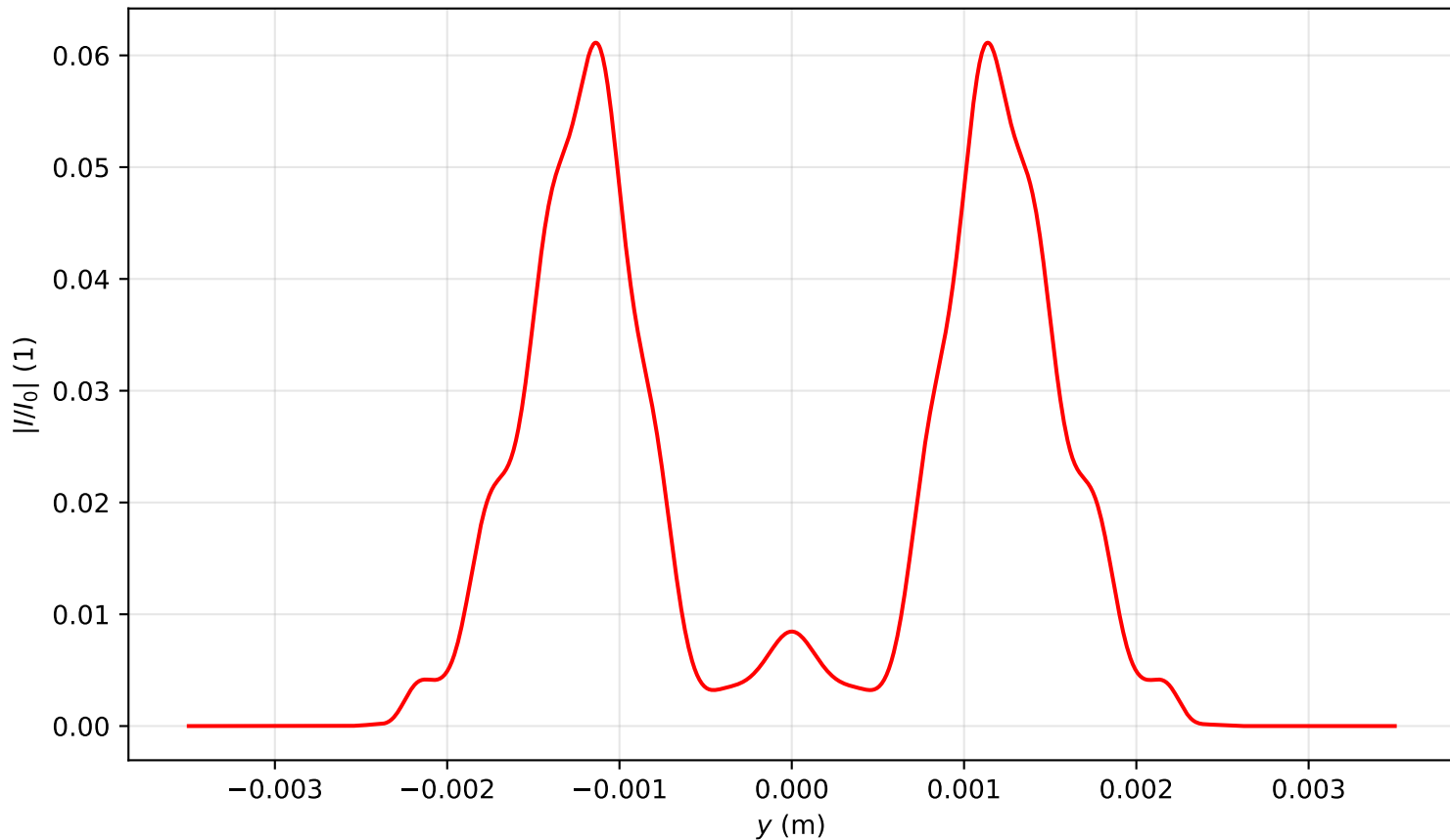
Intensity profile I(x=0, y, z=3.582)/I_0 , P_{in}=6.5P_{cr} , artificial time
